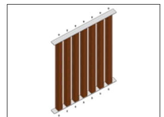
Top and Bottom Fixing
