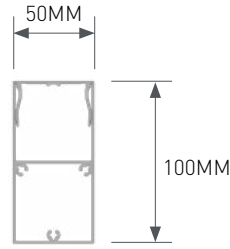
ALCL10050 - LOCK IN PROFILE
